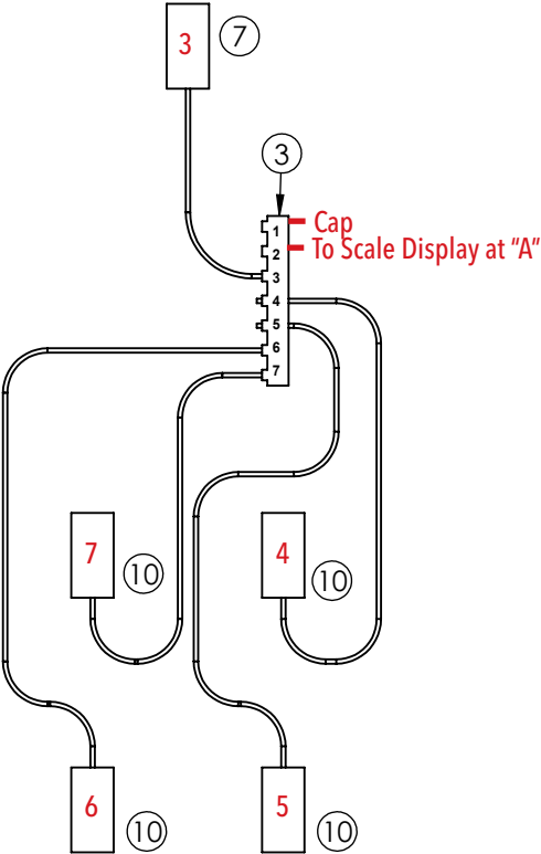
OPTIONAL REMOTE DISPLAY FOR 640M
