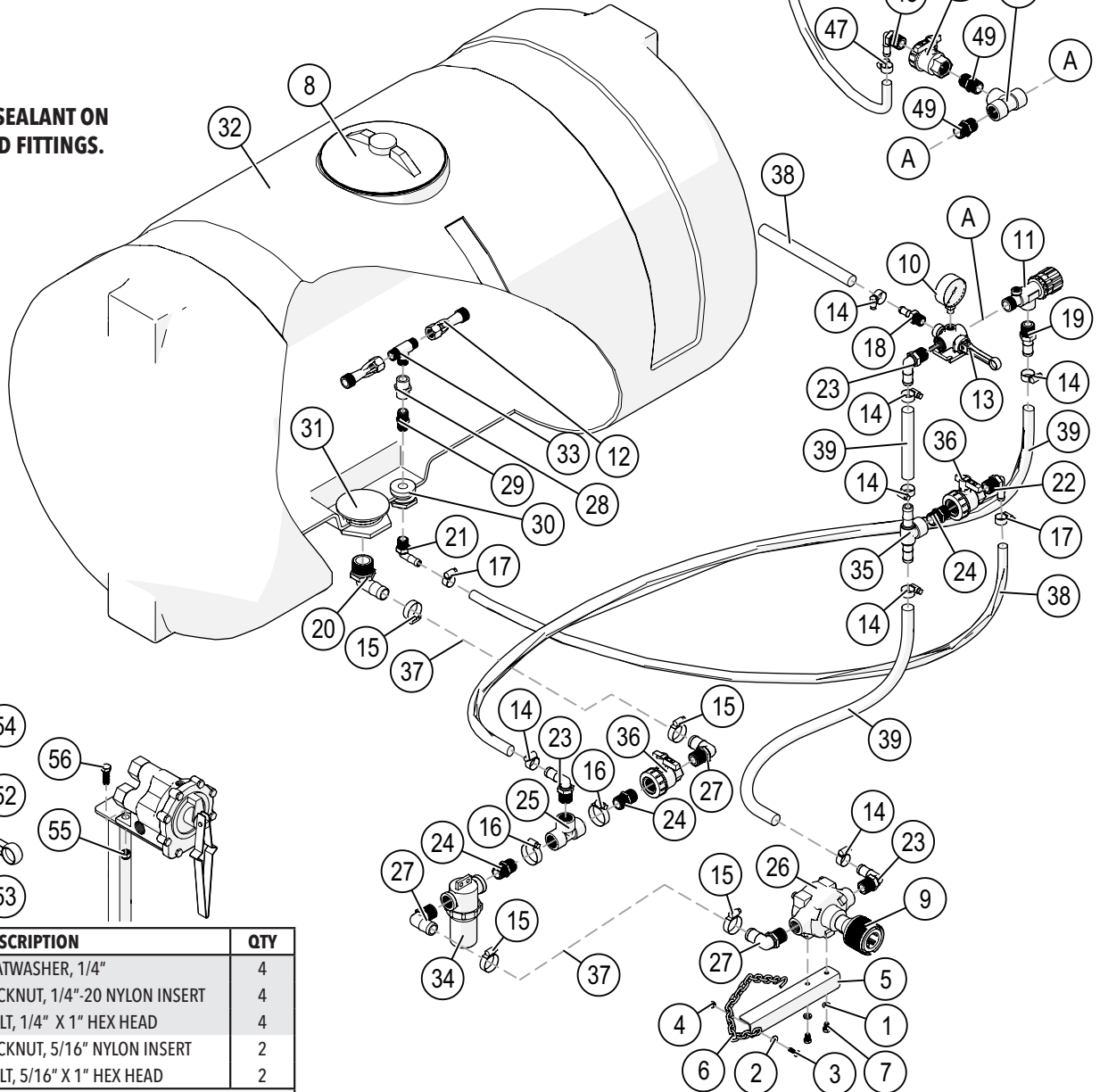
TRIPLE SECTION PLUMBING
