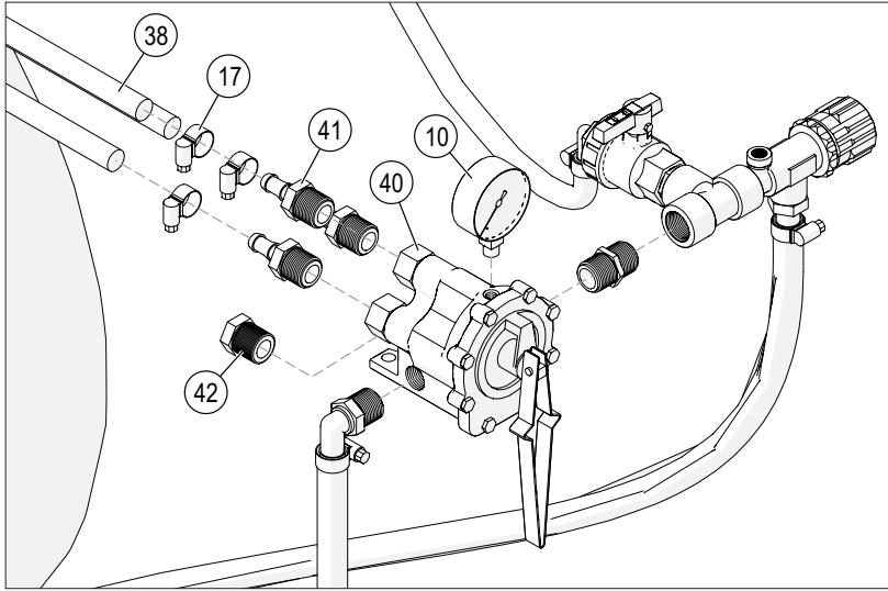
TRIPLE SECTION PLUMBING
