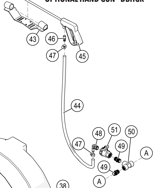
OPTIONAL HAND GUN - DBHGR
