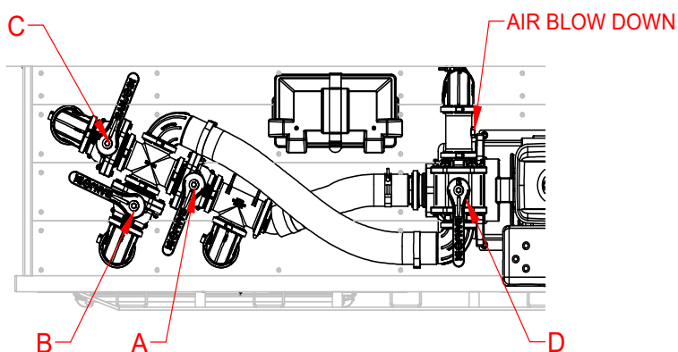
VALVE CLUSTER/FILL BANK VALVE DESIGNATION
