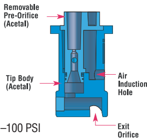
TTI110__VP SPRAY TIP (Cross Section View)
