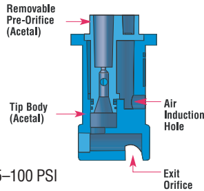
TTI110__VP SPRAY TIP (Cross Section View)
