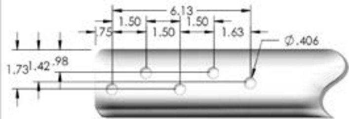
2" & 2 5/16" 50° A-Frame Mount
