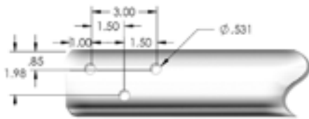
DA70 & DA86 Mount
