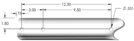
DA70 & DA86 Mount
