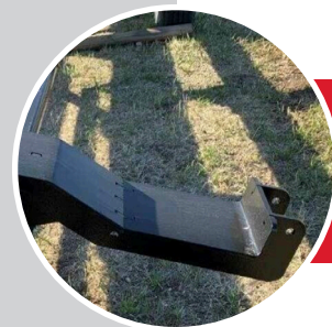
John Deere hinged draper feeder house brackets
